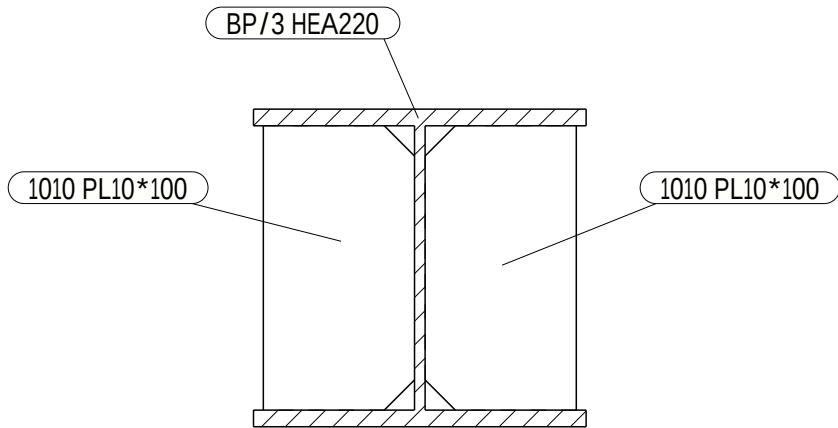
A - A 1:5
